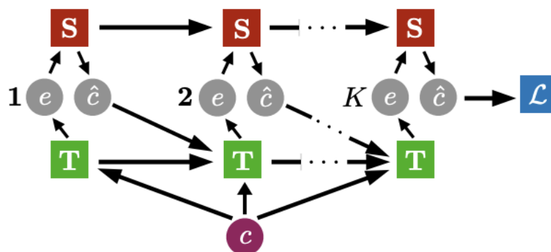
Figure 1. Visualization of Interpretability in Machine Learning based on Teacher-Student (T-S) interaction
