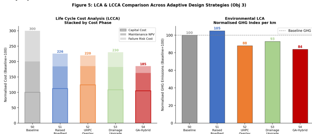
Figure 5: LCA & LCCA Analysis — Left: Stacked lifecycle cost by phase (capital, maintenance, failure risk). Right: Normalised GHG emission index. S4 achieves lowest total cost and lowest GHG.
