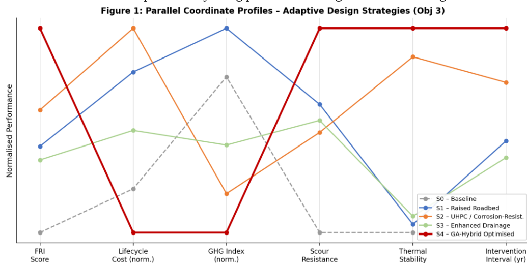
Figure 1: Parallel Coordinate Strategy Profiles — All five adaptive strategies (S0–S4) across six performance dimensions. S4 GA-Hybrid (red) dominates across the multi-dimensional space.
