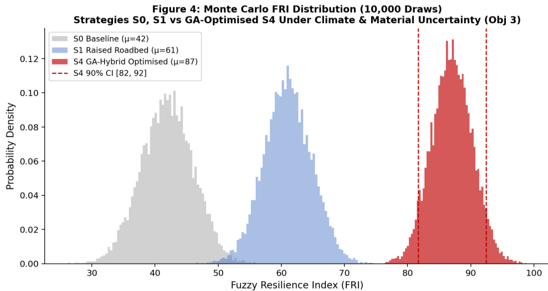
Figure 4: Monte Carlo FRI Distributions (10,000 draws) — S0 baseline (grey), S1 raised roadbed (blue), S4 GA-hybrid (red). S4 90% CI: [81, 93].
