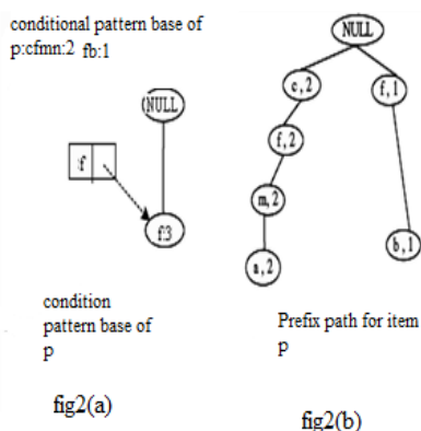
Figure 2: Prefix paths for Item
