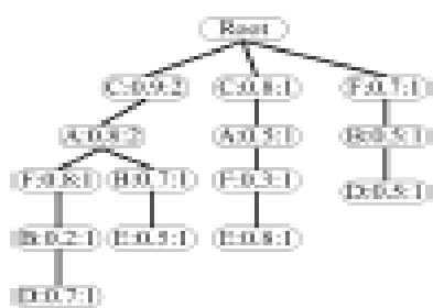
Figure 1: FP-Tree
