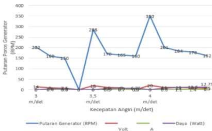
GRAPH 4.3. GRAPH OF WIND TURBINE TESTING WITH USING CONE TUNNEL
