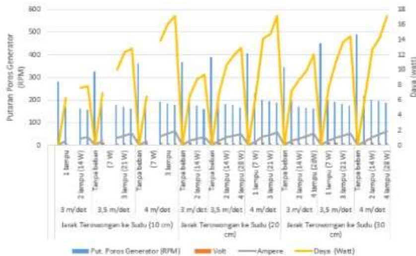
GRAPH 4.4. RELATIONSHIP BETWEEN TUNNEL DISTANCES – TO THE BLADE ON THE ROTATION AND THE POWER GENERATED
