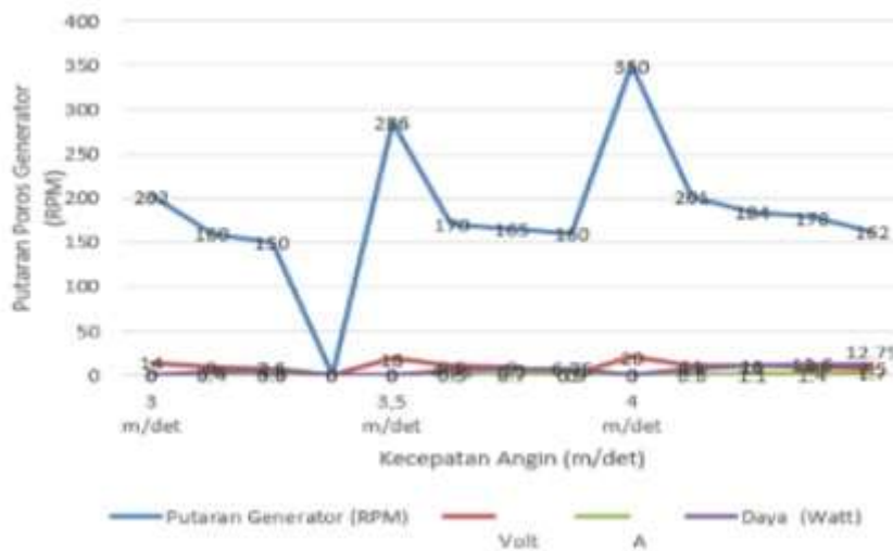
GRAPH 4.2. GRAPH OF WIND TURBINE TESTING WITHOUT USING CONE TUNNEL
