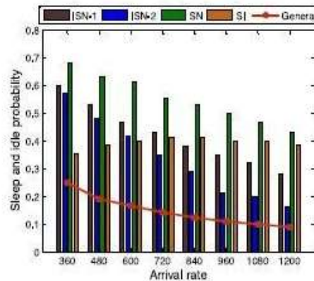
Figure 5.4 Policies arrival rate Analysis
