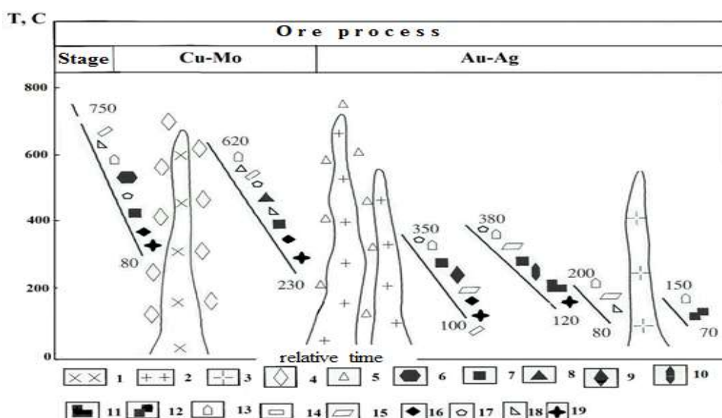
Fig. 3. Intra ore magmatism and sequence of ore formation Mekhmanian OMS (Volkov et al. , 2006 with the addition of the author).
