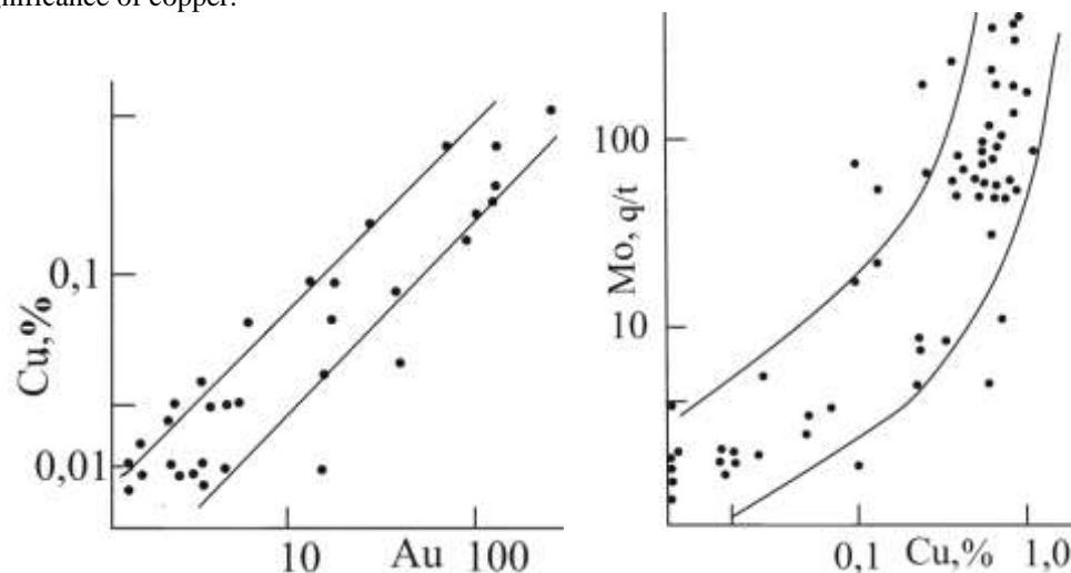
Fig.4. Dependence between the contents of copper, molybdenum and gold in the rocks of the Demirli deposit
