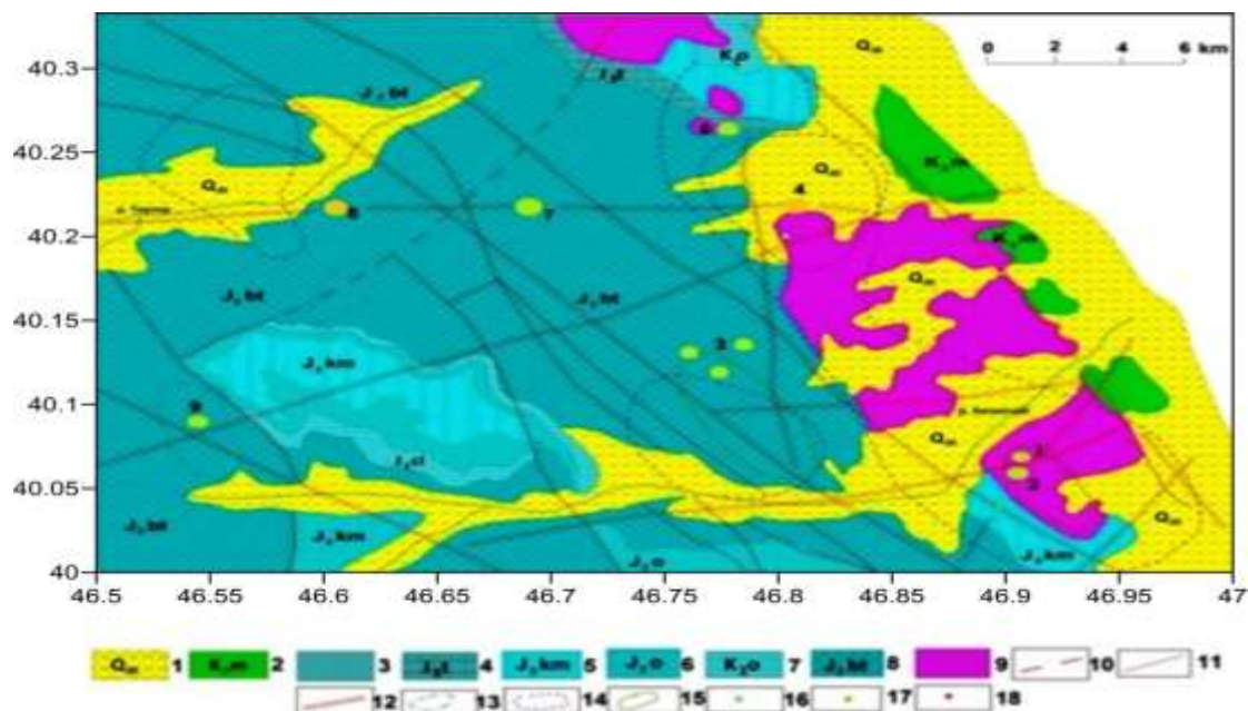
Fig. 1. Geological map of Mekhmanian ore district (Compiled on materials of Lesser Caucasian geological prospecting expedition)
