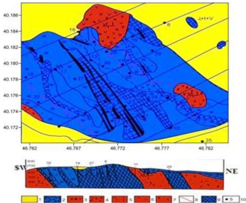
Fig. 2. Geological map Demirli deposit
